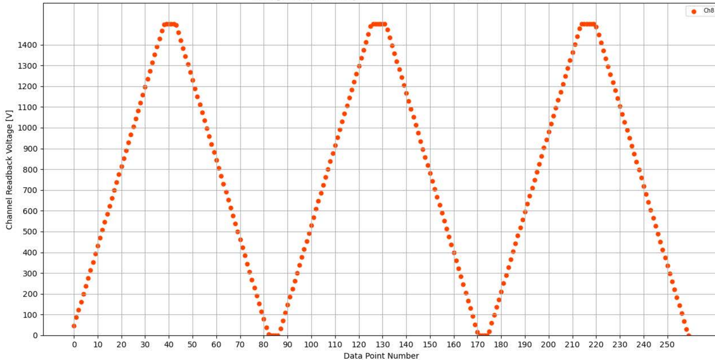
Voltage Ramp Test (Python) Bd #349, Slot #11, Ch #8
