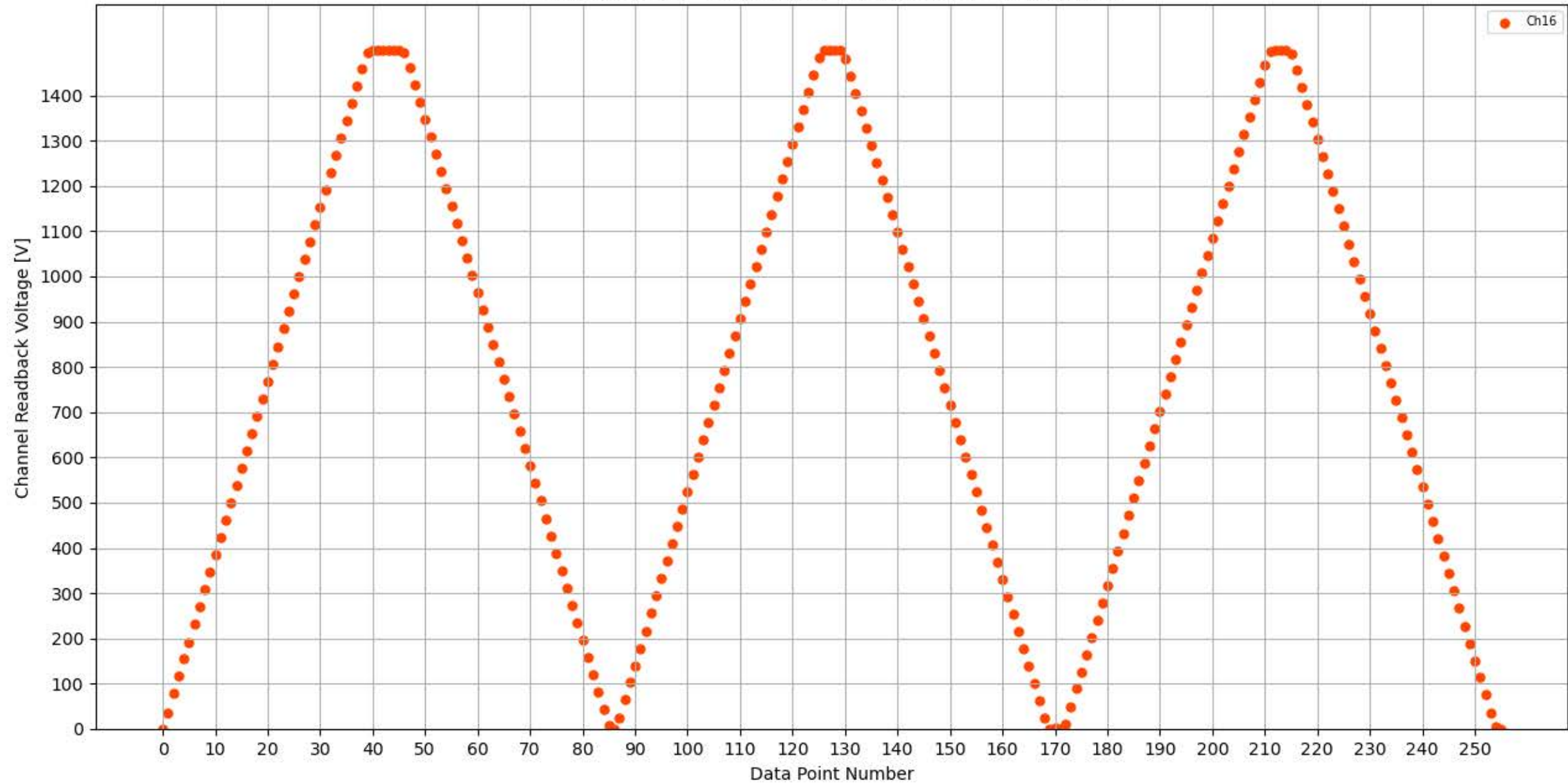
Voltage Ramp Test (Python) Bd #349, Slot #11, Ch #16
