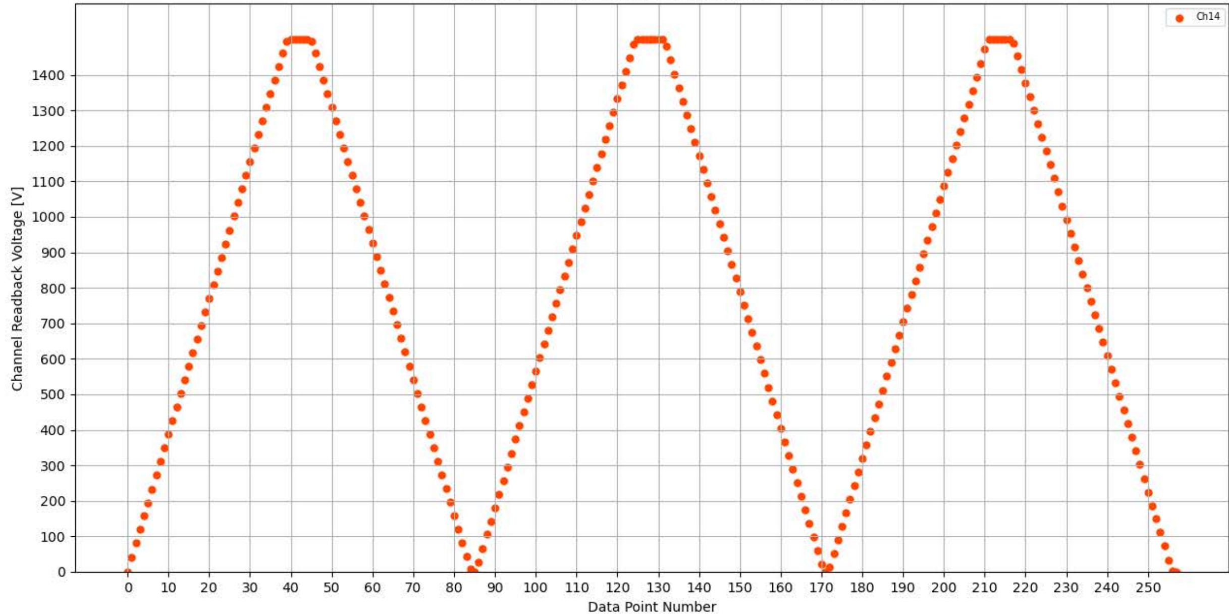
Voltage Ramp Test (Python) Bd #349, Slot #11, Ch #14
