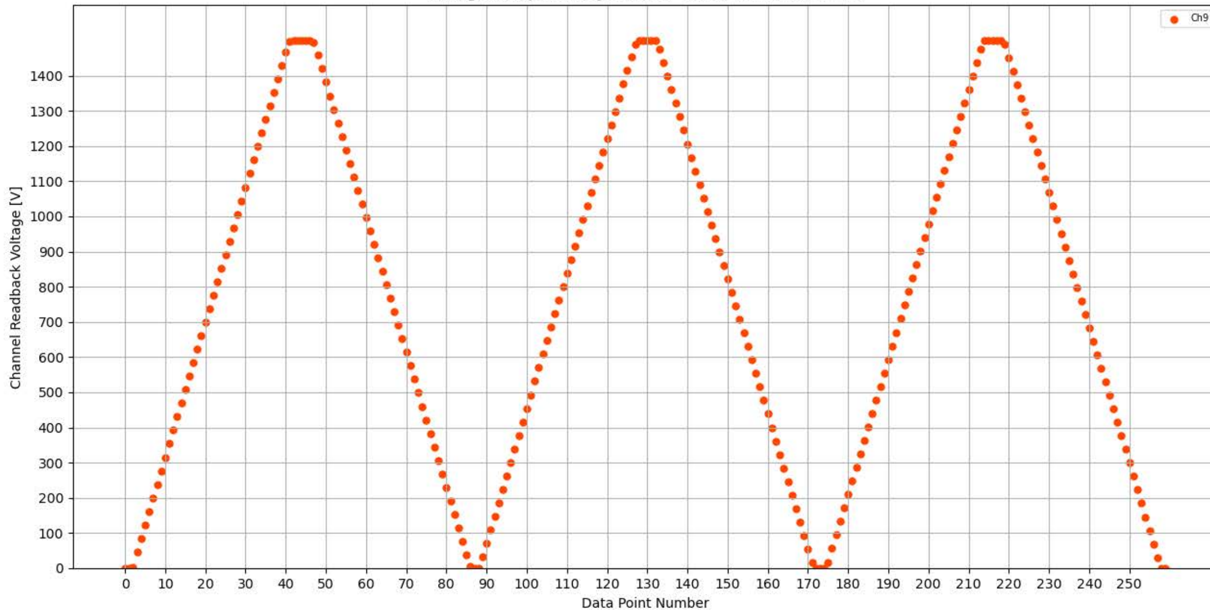
Voltage Ramp Test (Python) Bd #349, Slot #11, Ch #9
