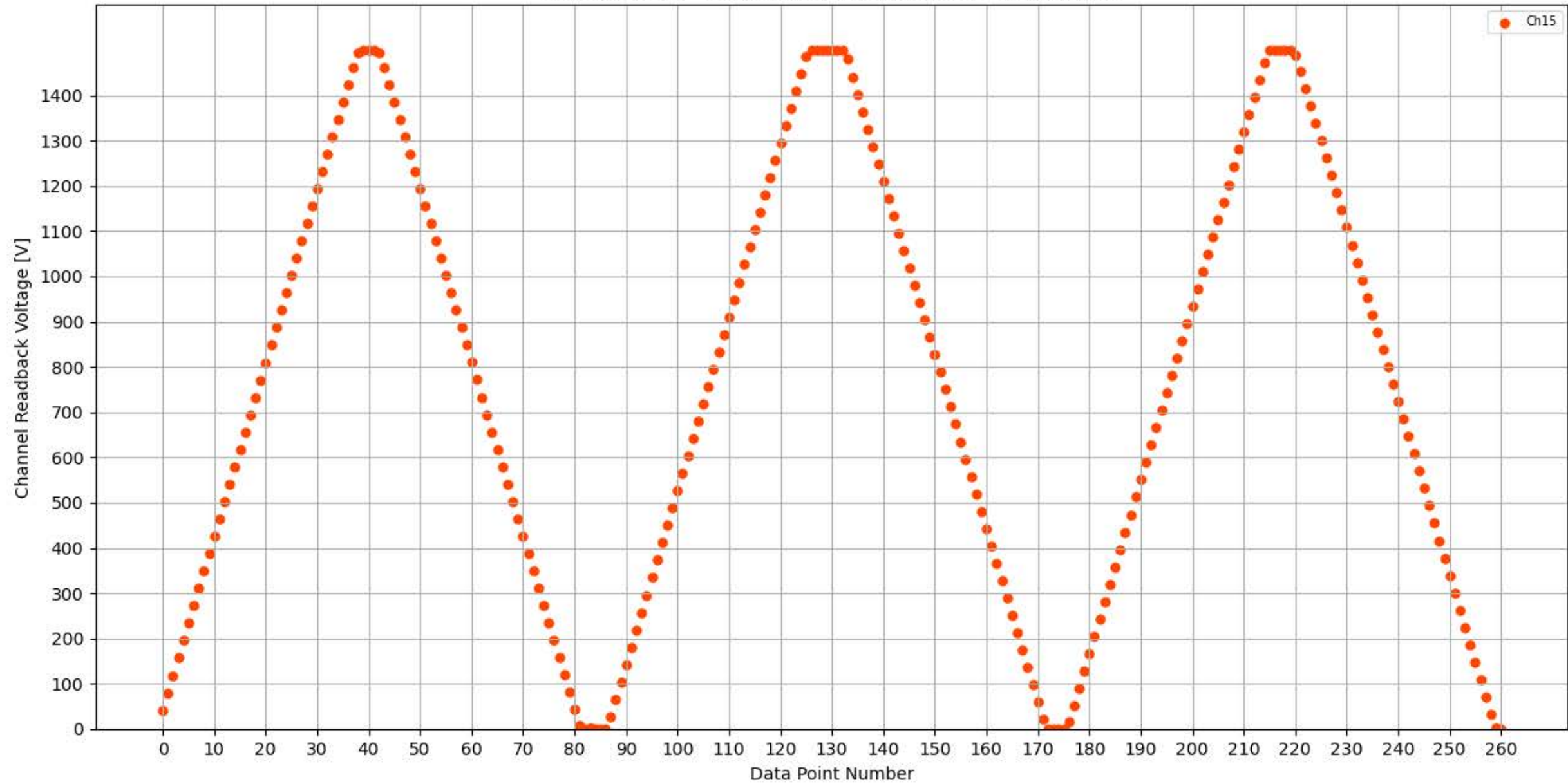
Voltage Ramp Test (Python) Bd #349, Slot #11, Ch #15
