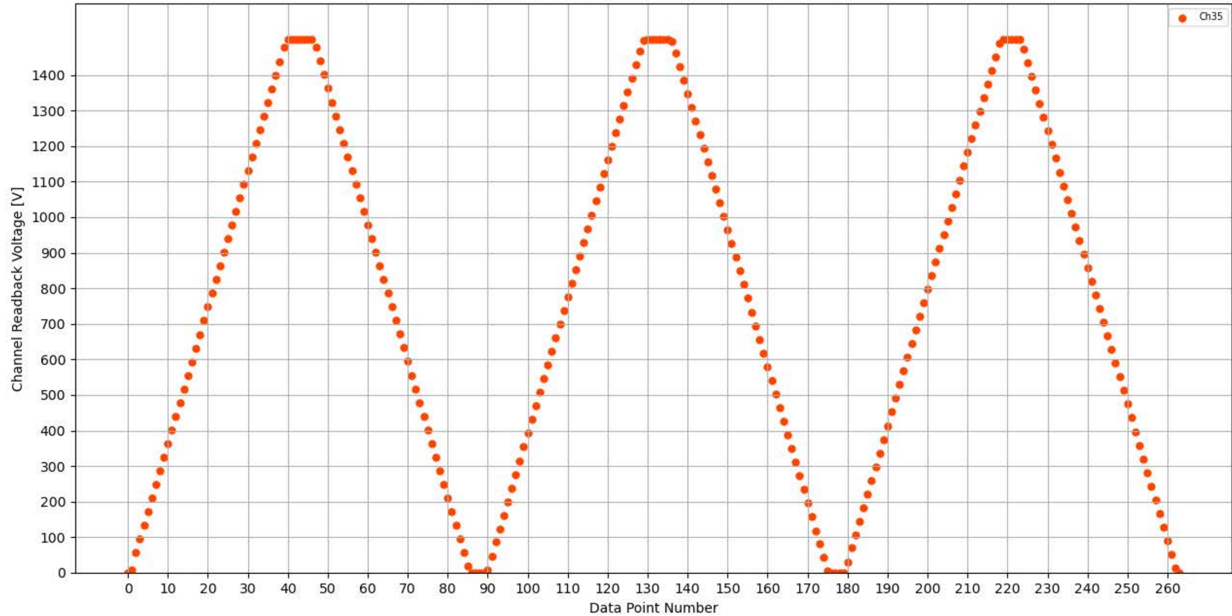
Voltage Ramp Test (Python) Bd #349, Slot #11, Ch #35
