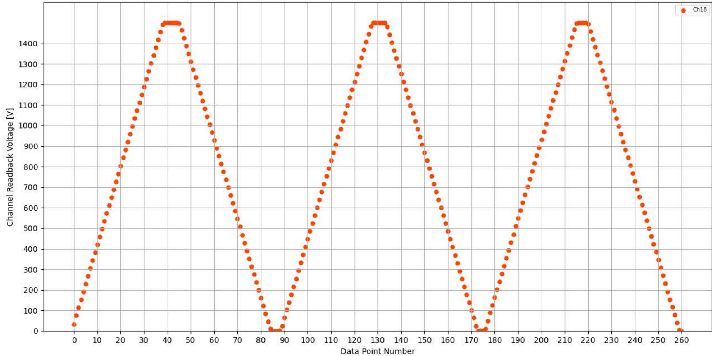
Voltage Ramp Test (Python) Bd #349, Slot #11, Ch #18
