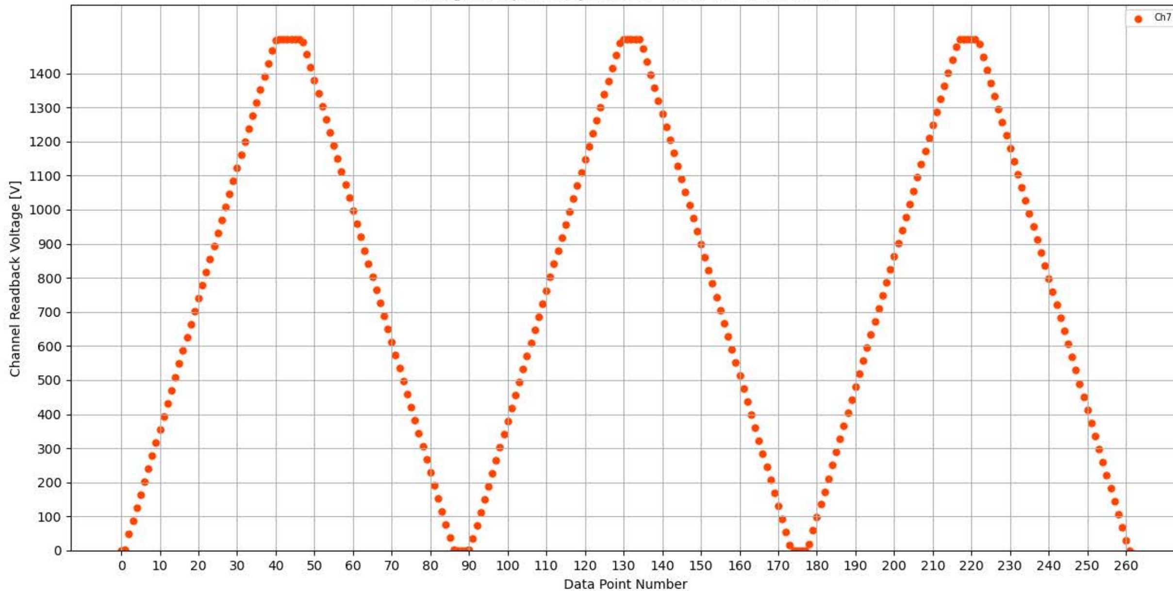
Voltage Ramp Test (Python) Bd #349, Slot #11, Ch #7
